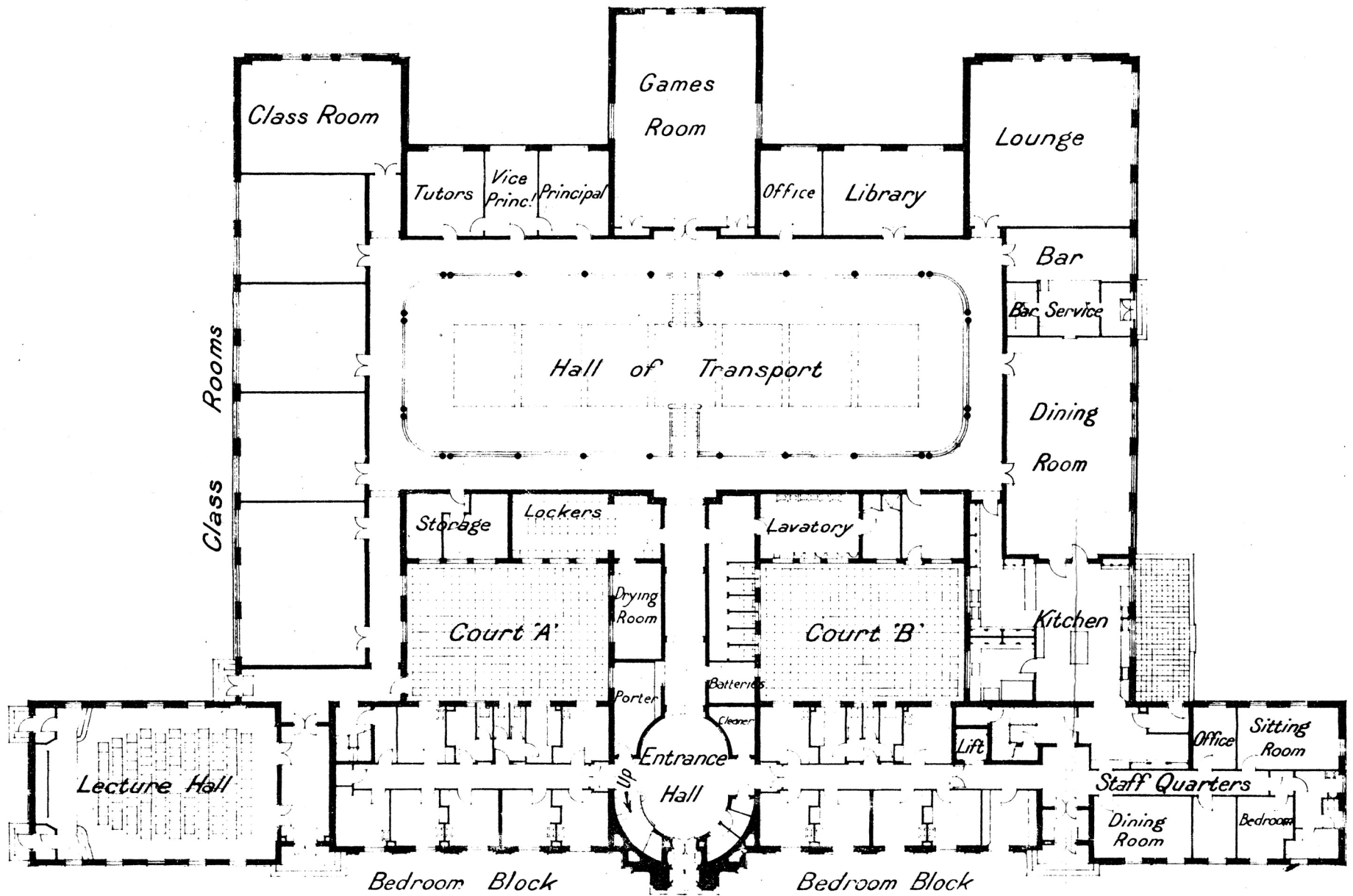
GROUND FLOOR
